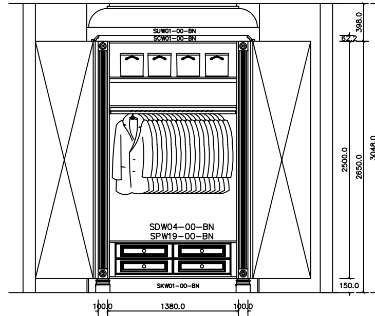
B VIEW
