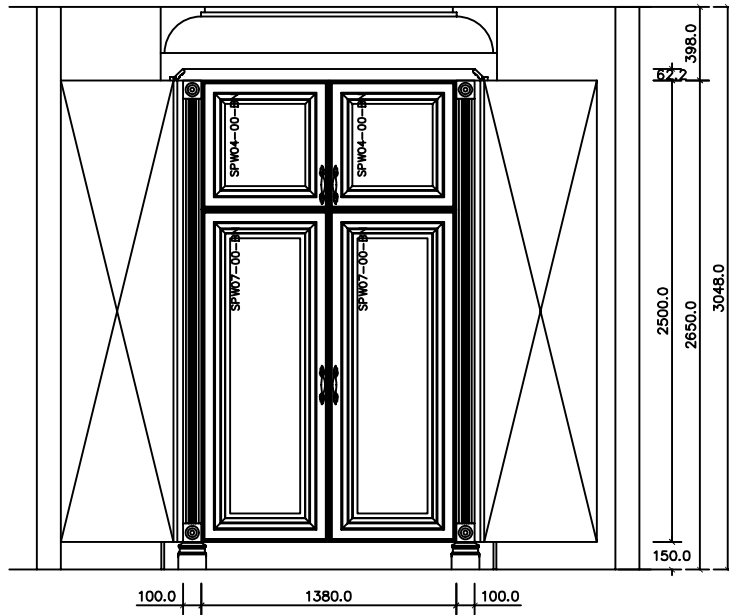
B VIEW
