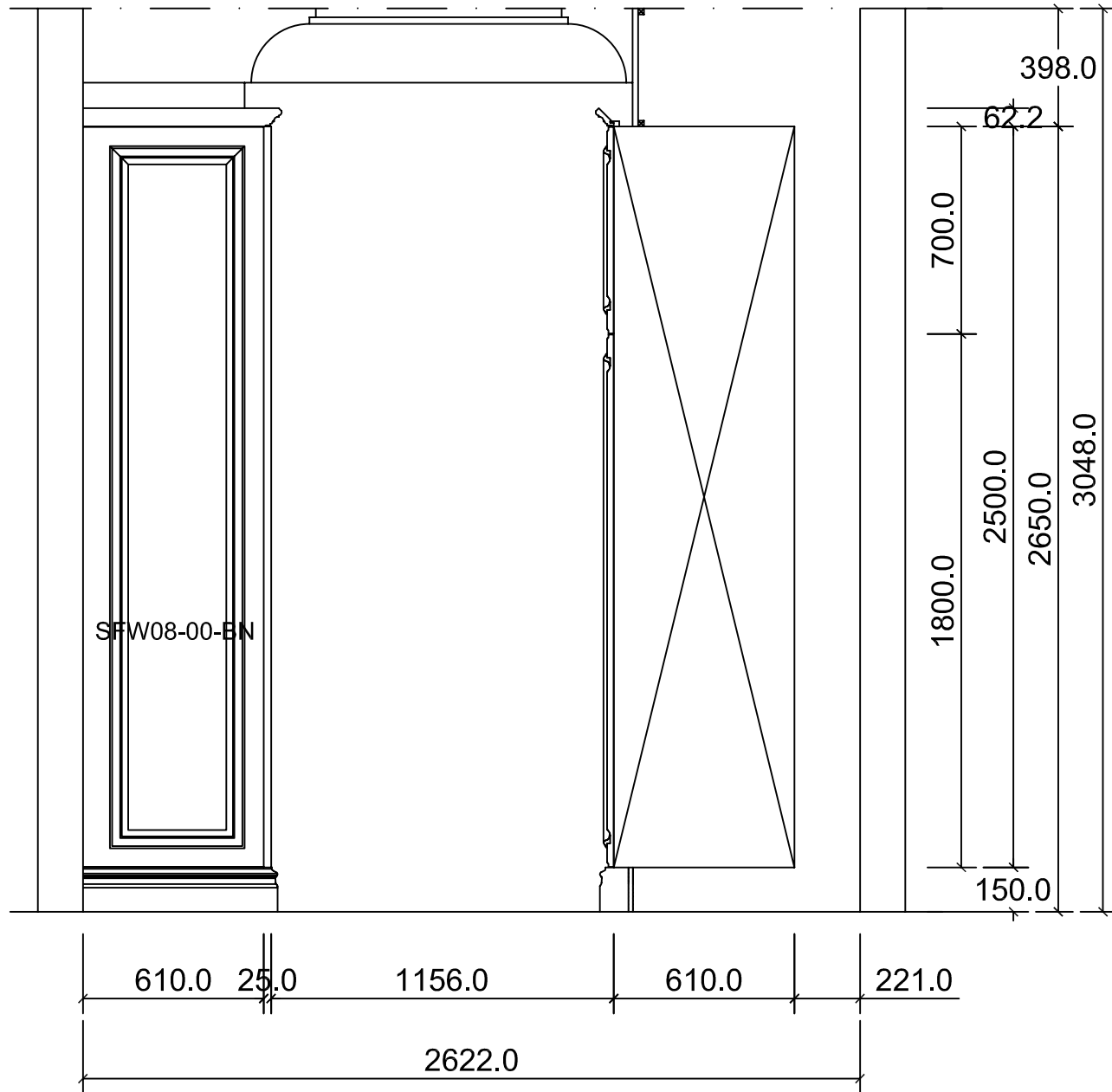
ELEVATION D
