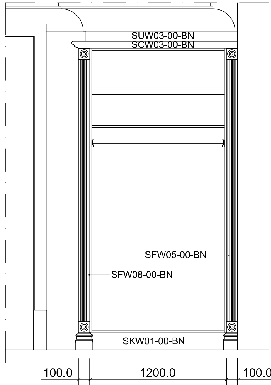
ELEVATION C
