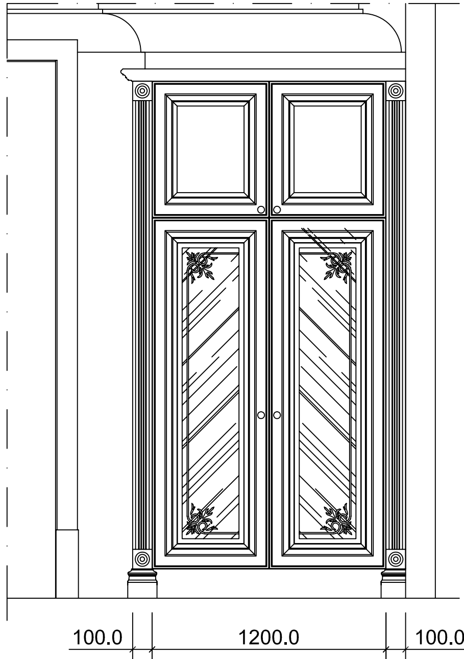
ELEVATION C
